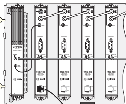
ethernet CAT-5E (crossover)
